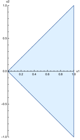
Figure 20: The set U_2
